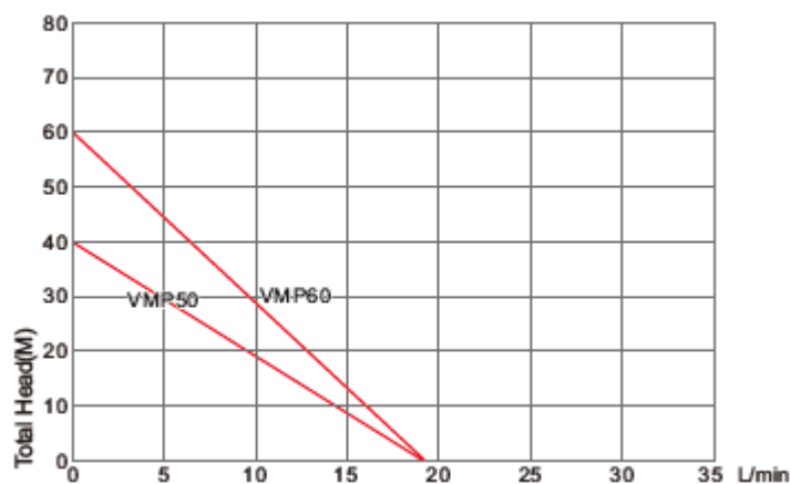
PERFORMANCE CHART AT n=2850\text{r/min}
